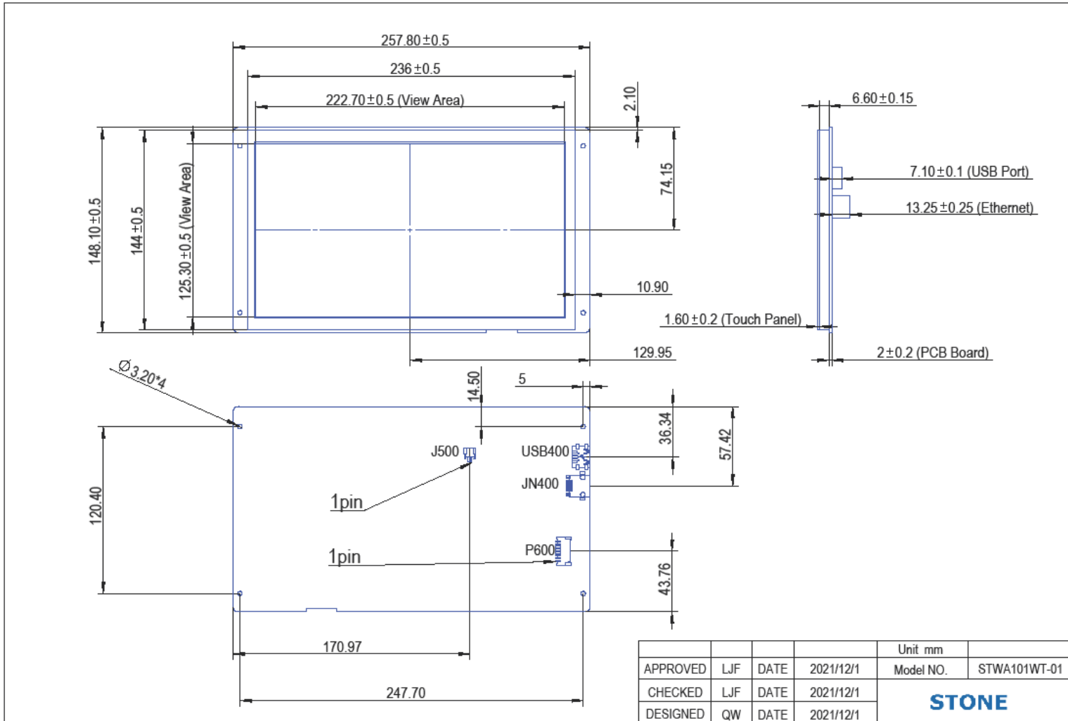
Figure 6-1 STWA101WT-01 dimension
